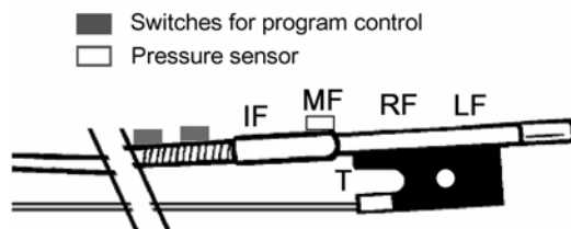
Figure 1. Positions of the (index-finger) switches and the middle-finger pressure sensor. All other bow-gesture sensors are mounted on a circuit board at the frog.
